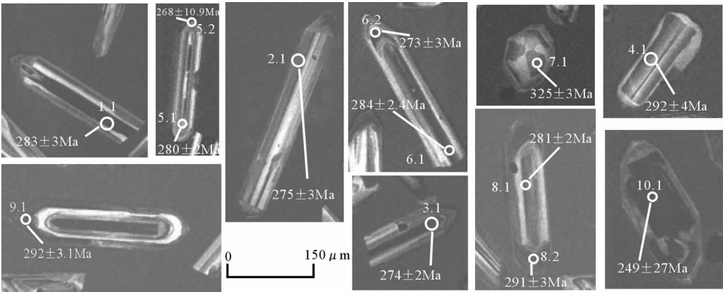
图 2 前进场岩体锆石阴极发光图像及各测点年龄 Fig.2 Cathodoluminescence images of zircons and ages of various analytical spots for the Qianjinchang granite
