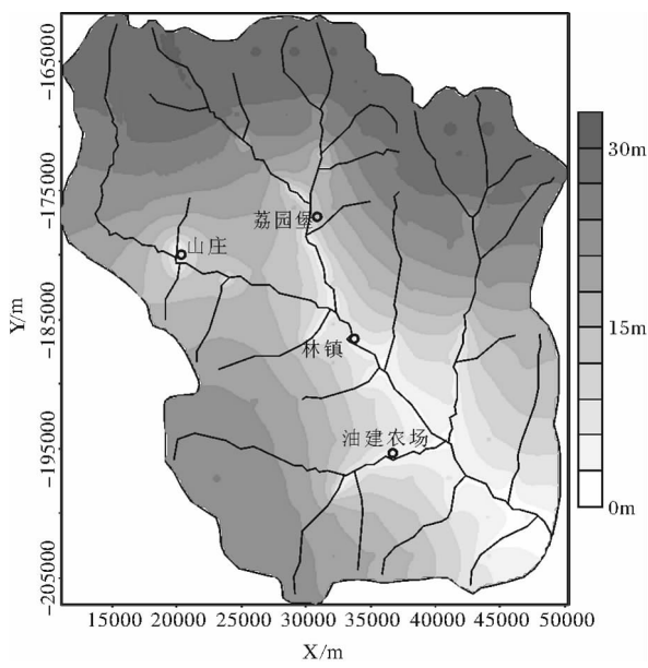
图 6 平均布井条件下降深分布 (开采量 35700 m 3 /d) Fig.6 Distribution of calculated steady state drawdown in an average well array scenario (yield 35700 m 3 /d)
