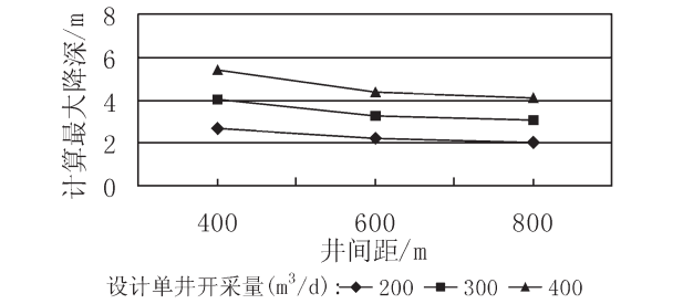
图 3 不同方案作用下井间距与计算最大降深关系曲线 Fig.3 Maximum drawdown—well spacing curves in different scenarios
