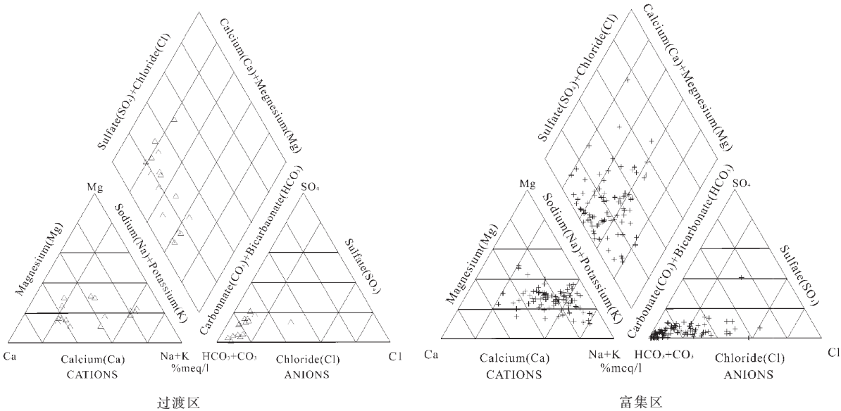
图 2 过渡区、富集区水化学类型 Fig.2 Hydrogeological types in transition and enrichment areas
