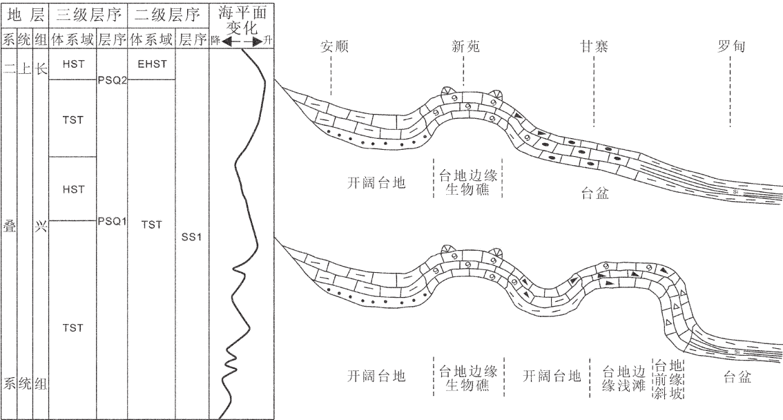
图 8 黔南拗陷长兴组沉积环境演化图 Fig.8 Sedimentary environment evolution diagram of Changxing Formation in southern Guizhou depression
