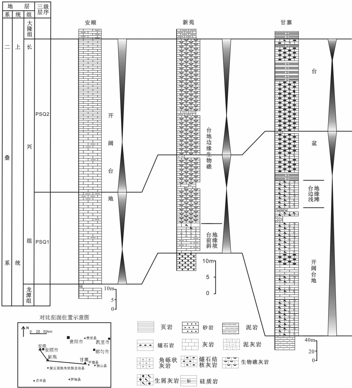
图 7 黔南坳陷上二叠统长兴组层序地层划分与对比图 Fig.7 Sequence stratigraphic division and comparison of Upper Permian Changxin Formation in southern Guizhou depression
