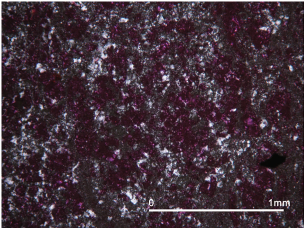
图 6 硅质岩, (正交偏光) Fig.6 Silicalite (Crossed nicols)
