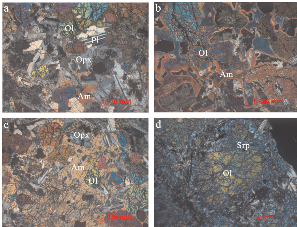
图2 红柳沟基性-超基性岩体矿物特征 a—橄榄角闪辉长苏长岩; b—橄榄辉长苏长岩中橄榄石的闪石次变边; c—橄榄角闪苏长岩中包含结构; d—辉石橄榄岩中橄榄石蛇纹石化; Ol—橄榄石; Opx—斜方辉石; Pl—斜长石; Am—角闪石; Srp—蛇纹石 Fig.2 Mineral characteristics of Hongliugou mafic-ultramafic complex a—Olivine hornblende gabbro norite; b— Amphibole kelyphite rim; c—Constraint structure; d—Serpentinized olivine; Ol—Olivine; Opx—Orthopyroxene; Pl—Plagioclase; Am—Amphibole; Srp—Serpentine
