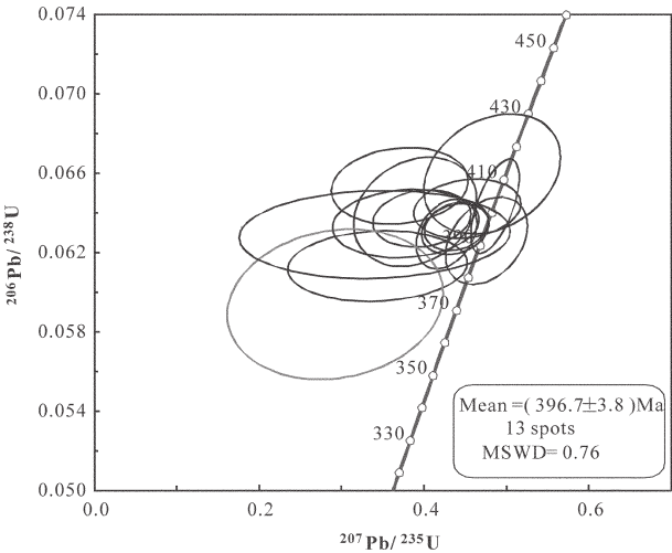
图5 红柳沟橄榄角闪辉长苏长岩锆石 U-Pb 谐和图 Fig.5 U-Pb concordia diagram of zircon from olivine hornblende gabbro norite of Hongliugou rock body
