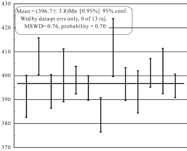
图6 红柳沟橄榄角闪辉长苏长岩锆石 206 Pb/ 238 U 年龄加权图 Fig.6 Weighted average 206 Pb/ 238 U age of zircon from olivine hornblende gabbro norite of Hongliugou rock body
