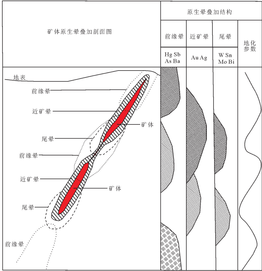
图6 娄里金矿体原生叠加晕模式示意图 Fig.6 Schematic diagram of primary superimposed halo model of the Louli gold deposit
