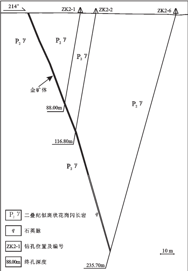
图4 图古日格金矿2-1号矿体2号勘探线剖面图 (据[16]修改) Fig. 4 Geological section along No. 2 exploration line of No. 2-1 orebody in the Tugurige gold deposit (modified after reference [16])
