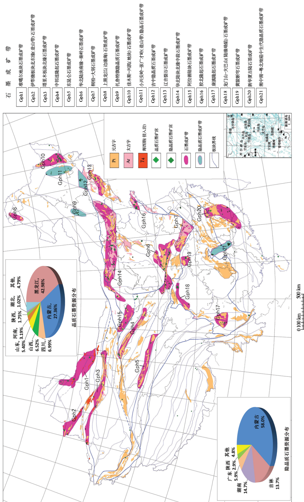
图5 中国石墨成矿带图 Fig.5 Metallogenic belts of graphite deposits in China
