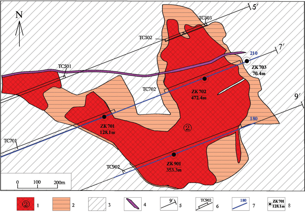
图8 ②号石墨矿体地质简图(据李作武等,2017) 1—石墨矿体及编号;2—细粒黑云母碱长花岗岩;3—中细粒黑云角闪碱长花岗岩;4—细粒花岗岩脉;5—勘探线剖面位置及编号; 6—探槽位置及编号;7—激电测深剖面位置及编号;8—见矿钻孔编号及孔深 Fig. 8 Geological sketch map of No. ② graphite orebody(after Li Zuowu et al., 2017) 1—Graphite orebody and its serial number; 2—Fine-grained biotite alkali-feldspar granite; 3—Medium fine-grained biotite hornblende alkali-feldspar granite; 4—Fine-grained granite dykes; 5—Exploration line section position and its serial number; 6—Trench position and serial number; 7—Excitation sounding section position and serial number; 8—Ore-intercepting drill hole and its serial number and depth
