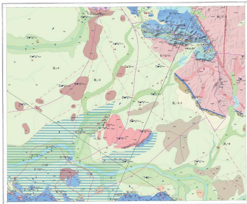
Fig. 2 1 : 50 000 Hydrogeological Map of Laiwu City
