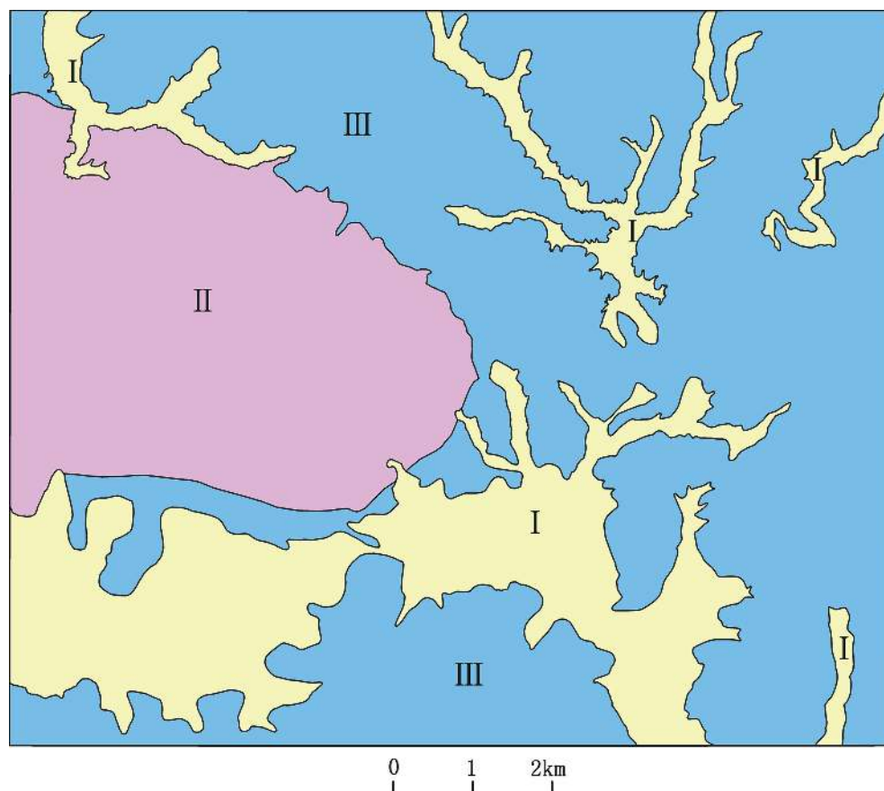
Fig. 3 Geological sub-area zoning in the Area
