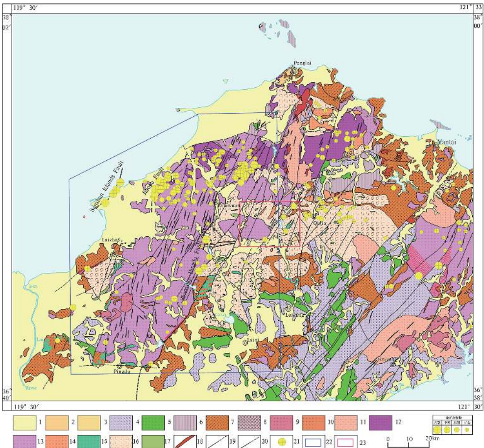
Fig. 1 Regional generalized geological map of the Shandong Zhaoyuan-Laizhou integrated exploration areaSchematic geological diagram
