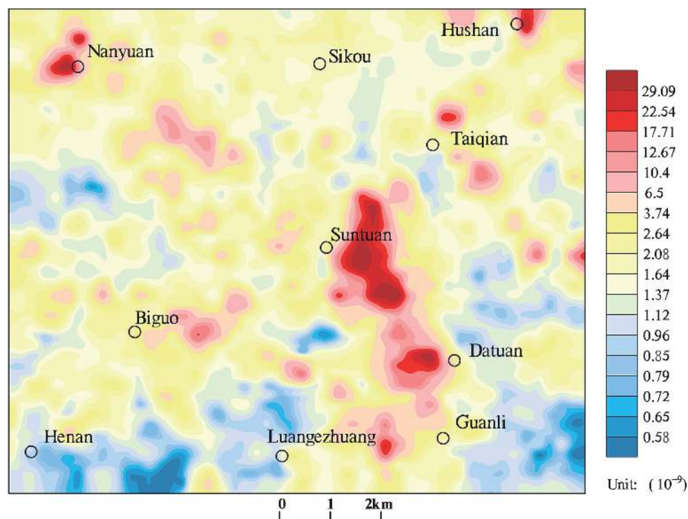
Fig. 2 Geochemical map of the element gold in the Area
