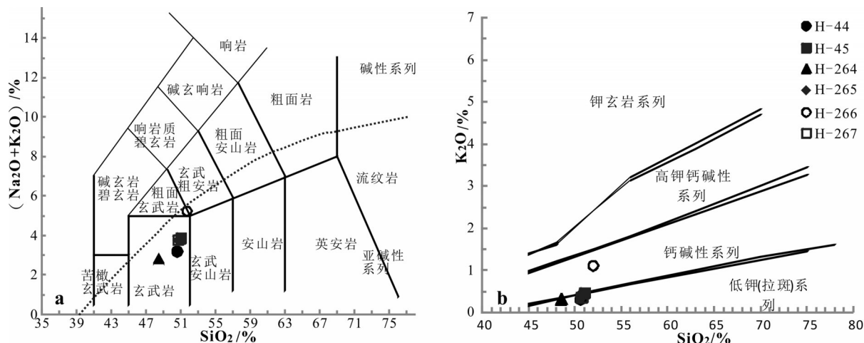
图3 黑石墩基性岩 TAS 图解(a)和 \text{SiO}_2 - \text{K}_2\text{O} 图解(b) Fig.3 TAS(a) and \text{SiO}_2 vs. \text{K}_2\text{O} (b) diagram of the Heishidun basic intrusive
