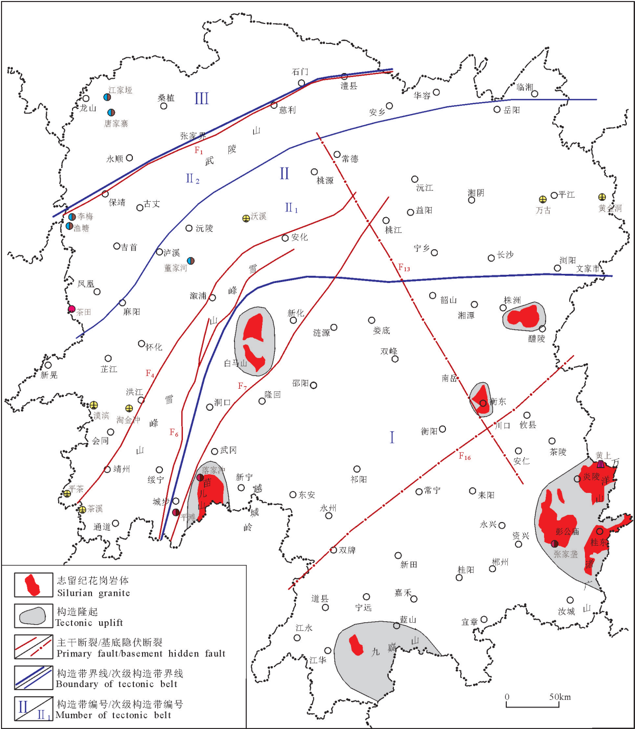
图2 志留纪后期内生热液成矿期构造格局(据柏道远等,2020;断裂名称及矿床类型同图1) I—湘中—湘东南构造岩浆带;II—雪峰构造带;II 1 —雪峰冲断带,II 2 —武陵低缓褶皱带;III—湘西北构造抬升带 Fig.2 Tectonic framework of late Silurian endogenous hydrothermal mineralization (after Bai Daoyuan et al., 2020; Names of faults and types of deposits same as fig.1) I—Central—Southeastern Hunan tectonomagmatic belt; II—Xuefeng tectonic belt; II 1 —Xuefeng thrust-fault zone; II 2 —Wuling gentle fold zone; III—Northwestern Hunan tectonic uplifting belt
