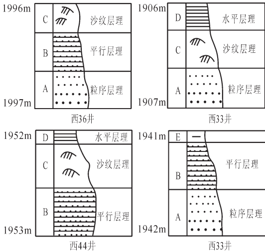
图4 鲍玛序列组合特征 Fig.4 Characteristics of the Bouma sequence
