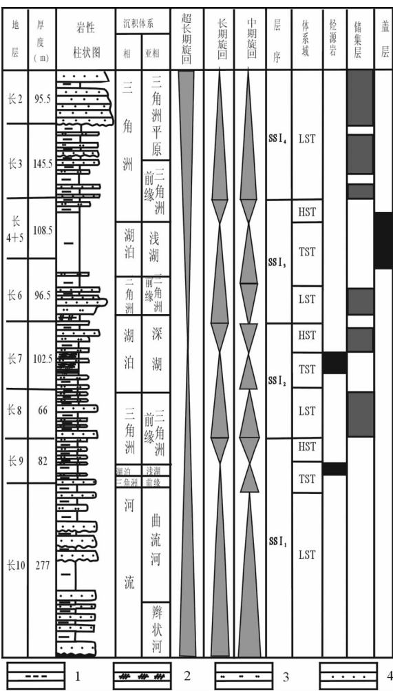
图 2 庆 36 井延长组沉积相-层序图 1—泥岩;2—油页岩;3—粉砂岩;4—细砂岩 Fig.2 Sedimentary facies and sequence stratigraphy of the Yanchang Formation in well Qing 36 1—Mudstone;2—Oil shale;3—Siltstone;4—Fine sandstone
