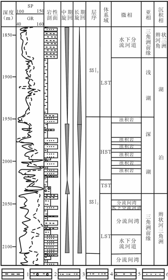
图3 西44井延长组层序地层—沉积相 1—泥岩;2—炭质泥岩;3—砂质泥岩;4—泥质砂岩; 5—粉砂岩;6—细砂岩 Fig.3 Sequence stratigraphy and sedimentary facies of Yanchang Formation from well Qing 44 1—Mudstone;2—Carbonaceous mudstone;3—Sandy mudstone; 4—Muddy sandstone; 5—Siltstone;6—Fine sandstone
