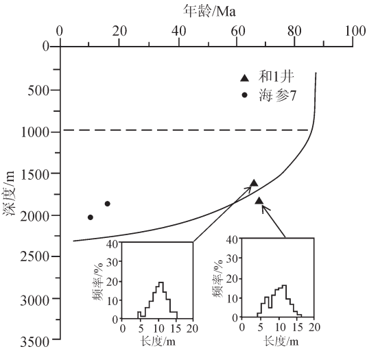
图 5 呼和湖凹陷磷灰石裂变径迹年龄与深度关系 Fig.5 Diagram of apatite fission-track ages vs. depths in the Huh Lake depression
