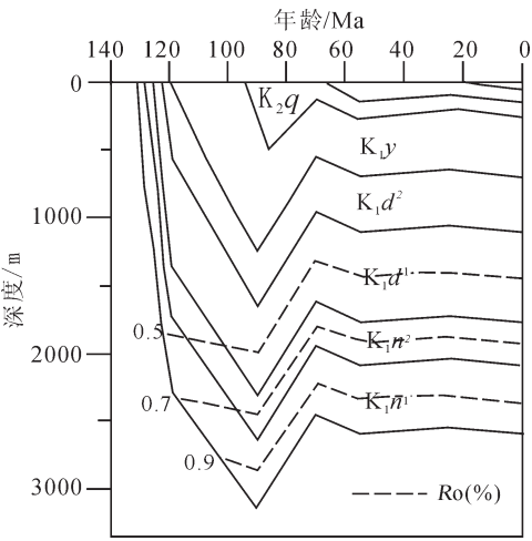
图 6 呼和湖凹陷热演化史与油气关系 K 2 q—青元岗组; K 1 y—伊敏组; K 1 d 2 —大磨拐河组上段; K 1 d 1 —大磨拐河组下段; K 1 n 2 —南屯组上段; K 1 n 1 —南屯组下段 Fig.6 Relation between the thermal history and oil-gas generation in the Huh Lake depression. K 2 q—Qingyuangang Formation; K 1 y—Yimin Formation; K 1 d 2 —Upper Member of the Damoguaihe Formation; K 1 d 1 —Lower Member of the Damoguaihe Formation; K 1 n 2 — Upper Member of the Nantun Formation; K 1 n 1 — Lower Member of the Nantun Formation
