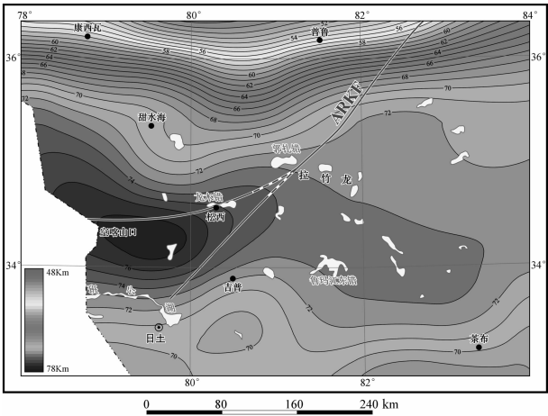
图 5 甜水海—郭扎错—日土一带的莫霍面等深度图 Fig.5 Moho depth map of the Tianshuihai-Gozha Co-Rutog area
