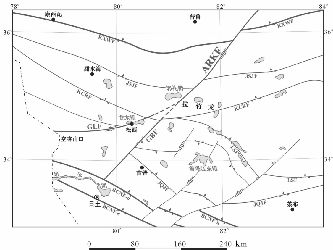
图 7 甜水海—郭扎错—日土一带断裂体系 ARKF—阿尔金断裂;GLF—郭扎错—龙木错断裂—班公湖断裂;GBF—郭扎错—班公湖断裂;BCNF-s—班公湖—怒江结合带南缘断裂;BCNF-N—班公湖—怒江结合带南缘断裂;JQJF—吉普—羌多—加错断裂;LSF—龙木错—双湖断裂;KCRF—克什尔村—楚沙尔—阿里坦廊断裂;JSJF—金沙江断裂;KXWF—康西瓦断裂 Fig.7 Fault system in the Tianshuihai-Gozha Co-Rutog area ARKF—Altyn Tagh fault;GLF—Gozha Co-Lungmu fault-Bangong Co fault;GBF—Gozha Co-Bangong Co fault;BCNF-S—Fault on the southern margin of the Bangong Co-Nujiang junction;BCNF-N—Fault on the northern margin of the Bangong Co-Nujiang junction;JQJF—Gyipug-Qangdoi-Gyaco fault; LSF—Lungmu Co-Shuanghu fault;KCRF—Keshen'er Village-Chusha'er-Alitanlang fault; JSJF—Jinshajiang fault;KXWF—Kangxiwar fault
