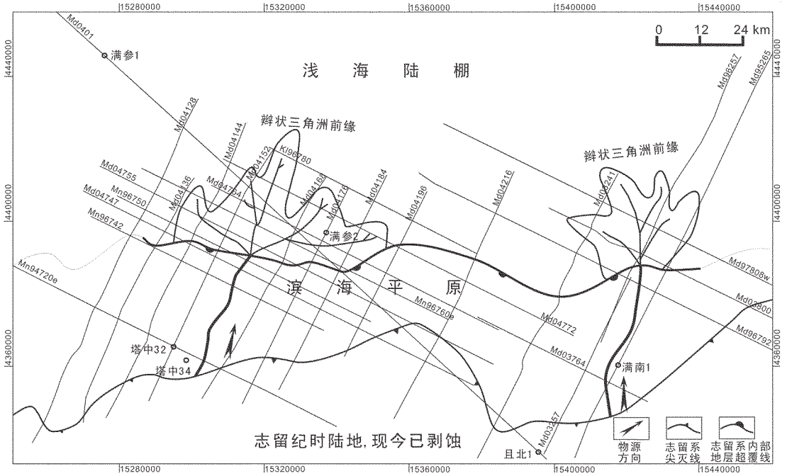
图7 满南地区志留系柯坪塔格组上段层序1低位域辫状三角洲前缘分布图 Fig.7 Distribution of braided-delta fronts in LST of sequence 1 in the Upper Member of the Silurian Kalpintag Formation in the southern Manjia'er subbasin
