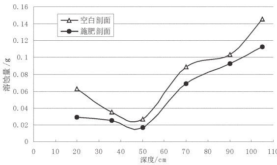
图 3 施肥与空白剖面石灰石溶蚀量对比 Fig.3 A comparison of the limestone dissolution in manure profile with that in control profile
