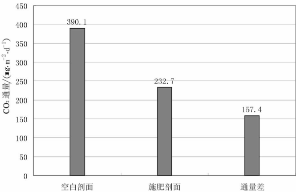
图 5 施肥与空白剖面地面 CO 2 通量对比 Fig.5 A comparison of the CO 2 flux in manure profile with that in control profile
