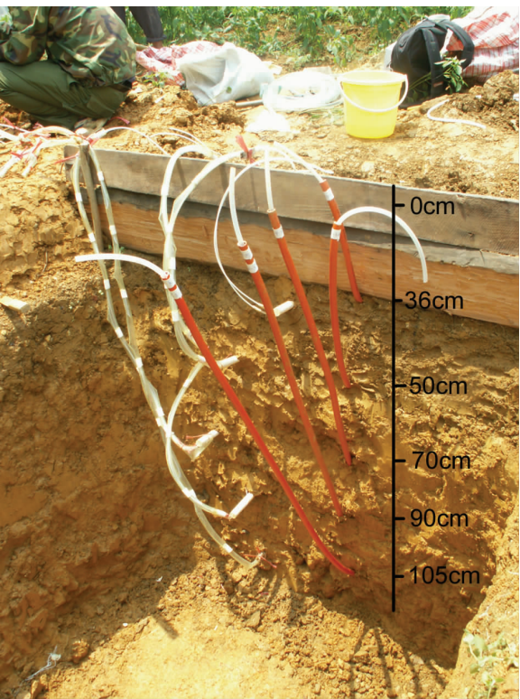
图 1 剖面土质及其影响因素观测 Fig.1 Observation of profile soil property and its affecting factors
