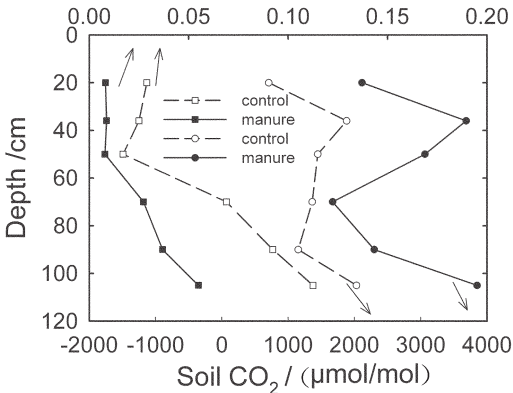
图 7 石灰岩溶蚀量与土壤 CO 2 浓度的关系 Fig.7 The relationship between the dissolution of limestone and soil CO 2
