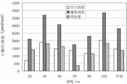
图 4 施肥与空白剖面土壤 CO 2 浓度及其对比 Fig.4 A comparison of the CO 2 concentration in manure profile with that in control profile
