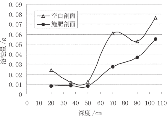
图 2 施肥与空白剖面白云石溶蚀量对比 Fig.2 A comparison of the dolomite dissolution in manure profile with that in control profile
