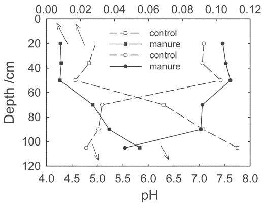
图 6 石灰岩年溶蚀量与 pH 的关系图 Fig.6 The relationship between the dissolution of limestone and soil pH
