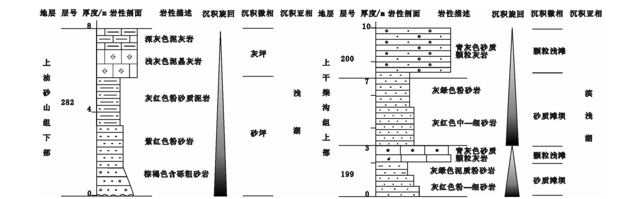
图 5 灰坪和颗粒浅滩沉积序列 Fig.5 Sedimentary sequence of calcareous flat and grain riffle
