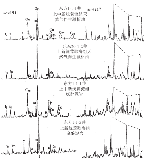
图8 莺歌海盆地泥底辟烃源岩与天然气伴生凝析油甾萜烷对比 Fig.8 Comparison between mud diapirs hydrocarbon rock and natural gas-associated condensate alkyl in Yingge Sea basin
