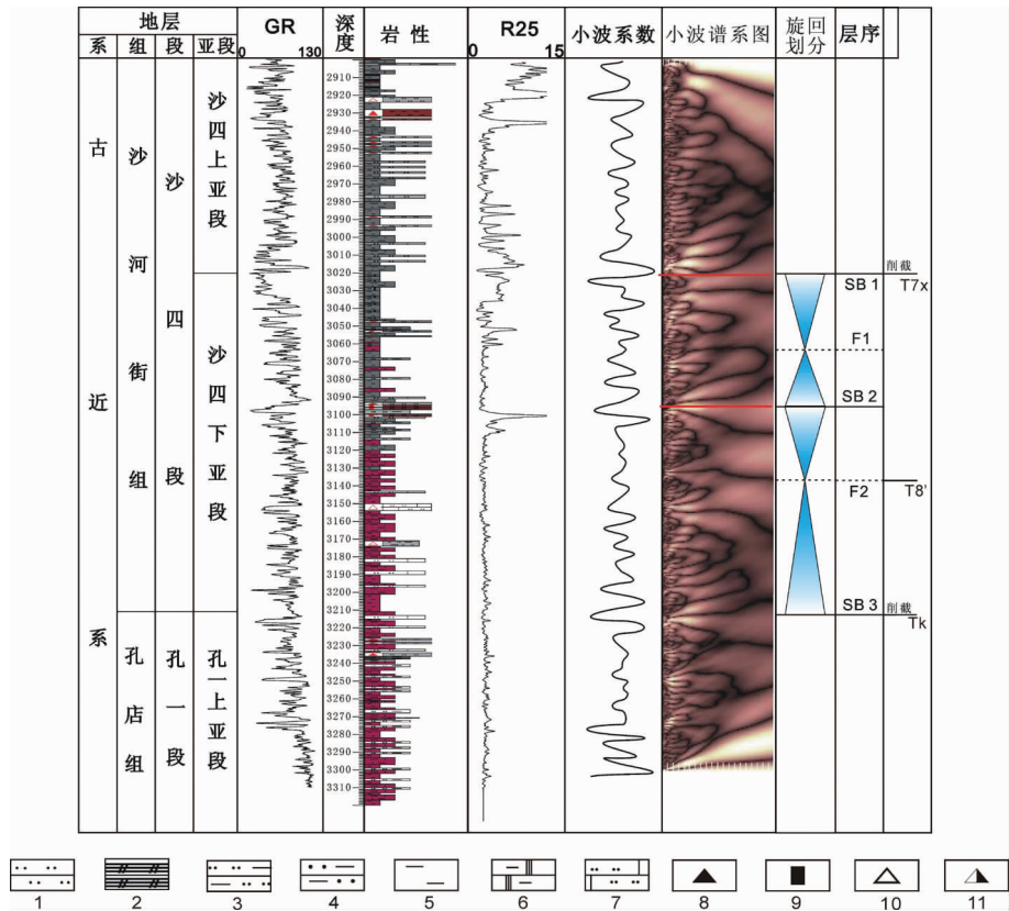
图 3 东营凹陷南坡沙四下亚段层序地层划分 1—砂岩;2—油页岩;3—砂质泥岩;4—泥质粉砂岩 5—泥岩;6—含石膏泥岩;7—灰质粉砂岩; 8—油斑;9—饱含油;10—油迹;11—荧光 Fig.3 Sequence stratigraphic division of Lower Es4 in the Dongying depression 1—Sandstone; 2—Oil shale; 3—Sandy mudstone; 4—Pelitic siltstone; 5—Mudstone; 6—Gypsiferous mudstone; 7—Cinereal siltstone; 8—Oil patch; 9—Oil-bearing grade of core; 10— Grease spot; 11—Fluorescence
