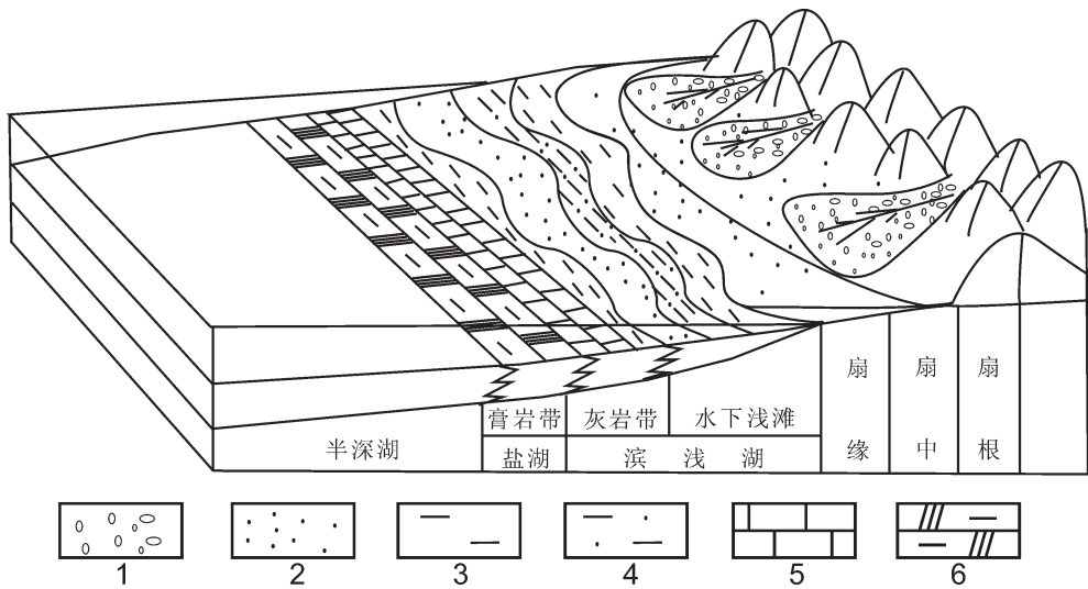
图 8 东营凹陷南坡沙四下亚段沉积充填模式图 1—砾岩;2—砂岩;3—泥岩;4—砂质泥岩;5—灰岩;6 膏岩 Fig.8 Sedimentary filling model of lower Es4 on the south slope of Dongying depression 1—Conglomerate; 2—Sandstone; 3—Mudstone; 4—Sand mudstone; 5—Limestone; 6—Gypsum rock
