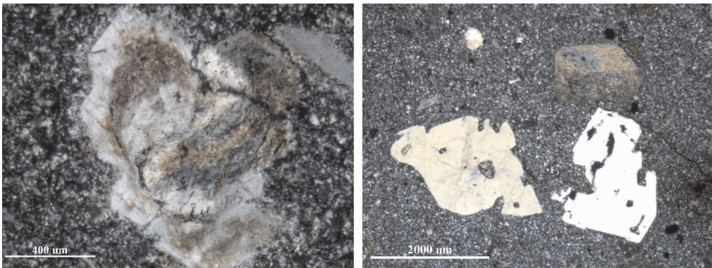
图 12 清水湾半岛白排湾粮船湾组碎斑熔岩显微照片(样品:08HK106) 左图:钾长石斑晶的碎斑结构,边部普遍发育珠边结构(正交偏光);右图:高温双锥状自形石英斑晶局部有熔蚀现象,流纹条带脱玻化形成霏细结构(正交偏光) Fig.12 Microphotographs of Kkh porphyroclastic lava at Pak Pai Wan of Clear Water Bay Peninsula (sample 08HK106) Left: K-feldspar phenocrysts have porphyroclastic structure and their margins commonly develops pearl-rim texture (crossed nicols); Right: Euhedral biconic quartz phenocrysts are corroded locally, and flow bandings were devitrified to form felsitic texture (crossed nicols)
