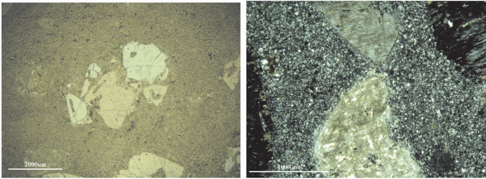
图 2 万宜水库南侧粮船湾组(Kkh)流纹质碎斑熔岩显微照片 左图:石英的碎斑结构与基质的流动构造(单偏光,样品 04HK-JW2);右图:钾长石斑晶的珠边结构 与基质的霏细结构(正交偏光,样品 04HK-JW3) Fig.2 Microphotographs of Kkh rhyolitic porphyroclastic lava at southern High Island Reservoir Left: Porphyroclastic structure of quartz and flow structure in the groundmass (plainlight, sample 04HK-JW2) Right: Pearl-rim texture of K-feldspar phenocrysts and felsitic texture in the groundmass(crossed nicils, sample 04HK-JW3)
