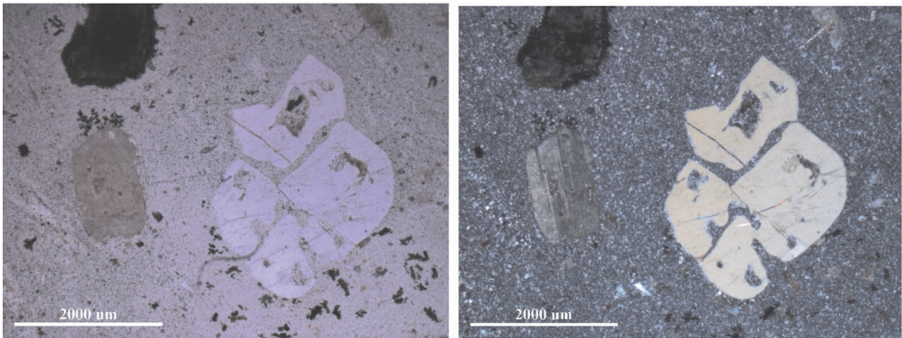
图 11 清水湾半岛白排湾粮船湾组碎斑熔岩显微照片(样品:08HK106) 左图:石英斑晶破碎,但仍保留其原始的双锥状形态;基质有明显流动构造(单偏光);右图:基质中细密的流纹条带普遍脱玻形成霏细结构,斜长石斑晶不发育珠边结构(正交偏光) Fig.11 Microphotographs of Kkh porphyroclastic lava at Pak Pai Wan of Clear Water Bay Peninsula (sample 08HK106) Left: Quartz phenocrysts are broken but preserve original biconic form, and the groundmass grows flow structure (plainlight); Right: Fine flow bandings in the groundmass were generally devitrified and formed felsitic texture, pearl-rim texture is poorly developed in plagioclase phenocrysts (crossed nicols)
