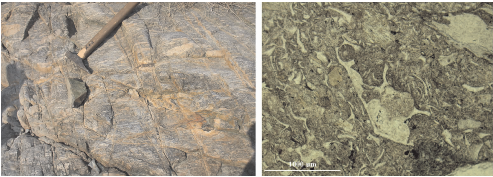
图 19 浙江宁波馆头组强熔结凝灰岩 (左) 和泰顺西山头组玻屑凝灰岩显微结构 (右) 左图: 熔结凝灰岩露头清晰可见大量定向排列的灰白色浆屑条带; 右图: 玻屑凝灰岩含丰富刚性玻屑, 部分较大的玻屑保留较完整气孔 (单偏光, 样品 O6TS-09) Fig.19 Guantou Formation strongly welded tuff in Ningbo (left) and Xishantou Formation vitric tuff in Taishun (right), Zhejiang Province Left: Lots of dark grey oriented fiammes are exposed on the surface of welded tuffs; Right: Vitric tuff contains plentiful vitric fragments which have individual vesicles (plainlight, sample 06TS-09)
