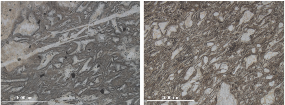
图 20 熔结凝灰岩中不同程度变形的塑性玻屑 (产地: 浙江) 左图: 弱熔结凝灰岩, 塑性玻屑变形较弱, 略有压扁定向排列 (单偏光, 样品: D084); 右图: 强熔结凝灰岩, 塑性玻屑强烈压扁拉长定向排列, 但其形态仍清晰可辨 (单偏光, 样品: D094-2) Fig.20 Plastic vitric fragments with different weldings in welded tuffs (from Zhejiang Province) Left: Weakly-welded tuff contains weakly deformed and insignificant oriented plastic vitric fragments (plainlight, sample D084); Right: Strongly-welded tuff contains strongly flattened and oriented plastic vitric fragments (plainlight, Sample D094-2)
