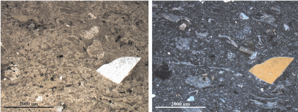
图 17 清水湾半岛碧沙湾鸕鸕山组(Krc)流纹质熔结凝灰岩显微照片(样品 08HK2-1) 左图:压扁拉长的浆屑和塑性玻屑形态可辨,石英和长石晶屑均呈棱角状(单偏光);右图:脱玻化的浆屑和塑性玻屑之形态因绢云母化而更显清晰,构成假流动构造(正交偏光) Fig.17 Microphotographs of Krc rhyolitic welded tuff at Bayside Beach of Clear Water Bay Peninsula (sample 08HK2-1) Left: Oriented flattened fiammes and plastic vitric fragments are clear, quartz and feldspar fragments are all angular(plainlight); Right: Devitrified fiammes and plastic vitric fragments were all sericitized and formed pseudo-rhyolitic structure (crossed nicols)
