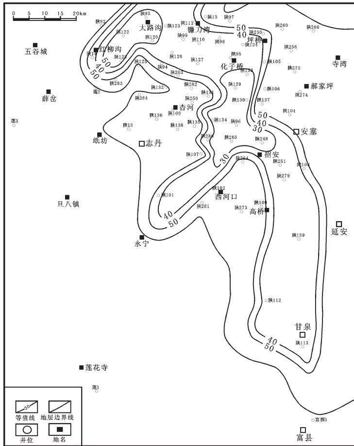
图 3 靖边潜台南部奥陶系马五 2 准同生白云岩含量(%)等值线图 Fig.3 Contour map of para-contemporaneous dolostones content (%) of Ordovician Ma5 2 in southern Jingbian tableland
