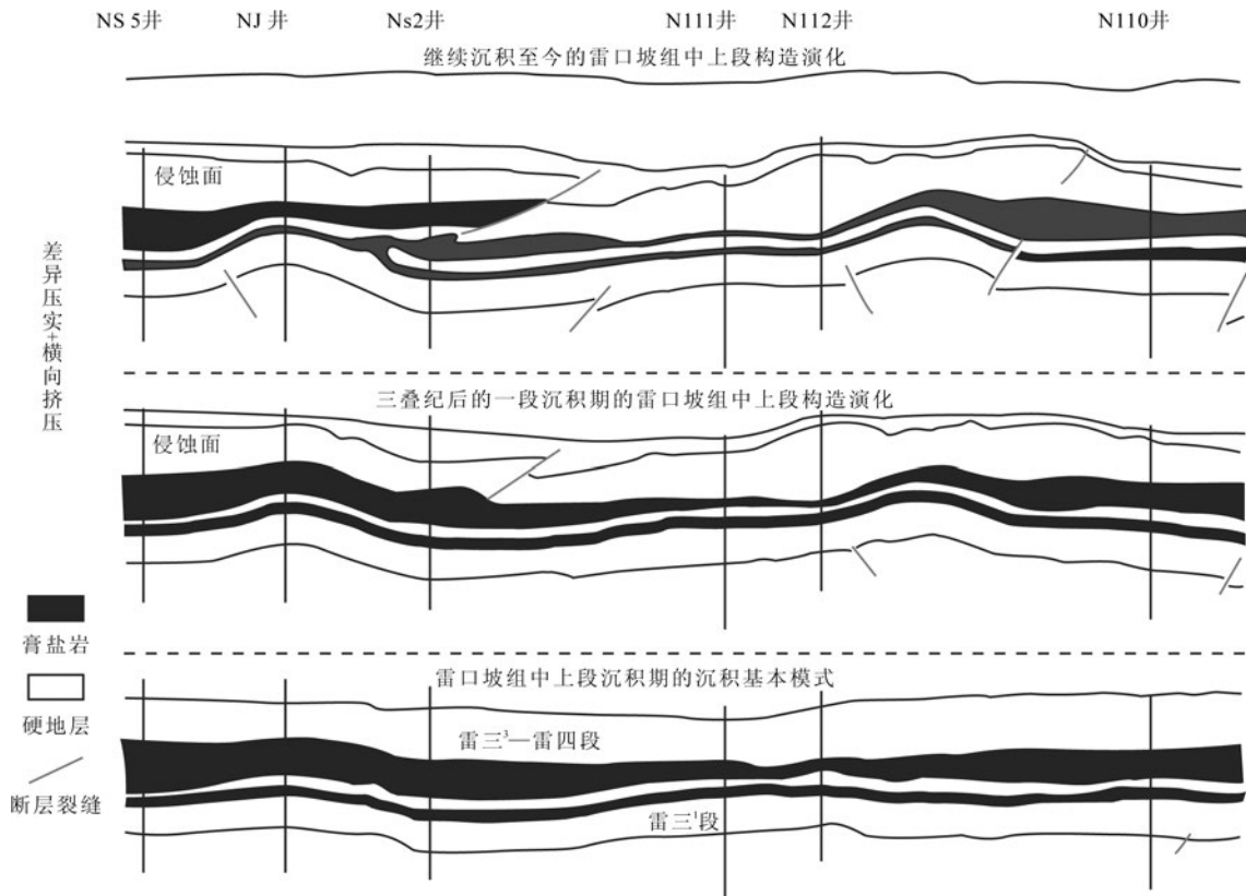
图5 川中南部龙女寺地区的雷口坡组中上部地层沉积和构造演化示意图(据文献[40]修改) Fig.5 Sedimentary and tectonic evolution diagram of upper strata of Leikoupo Formation in Longnvsi area of southern central Sichuan basin(modified after Reference[40])
