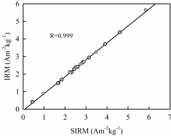
图 2 高砷含水层沉积物样品中饱和等温剩磁与等温剩磁关系图 Fig.2 The relationship between SIRM and IRM of high arsenic aquifer sediments
