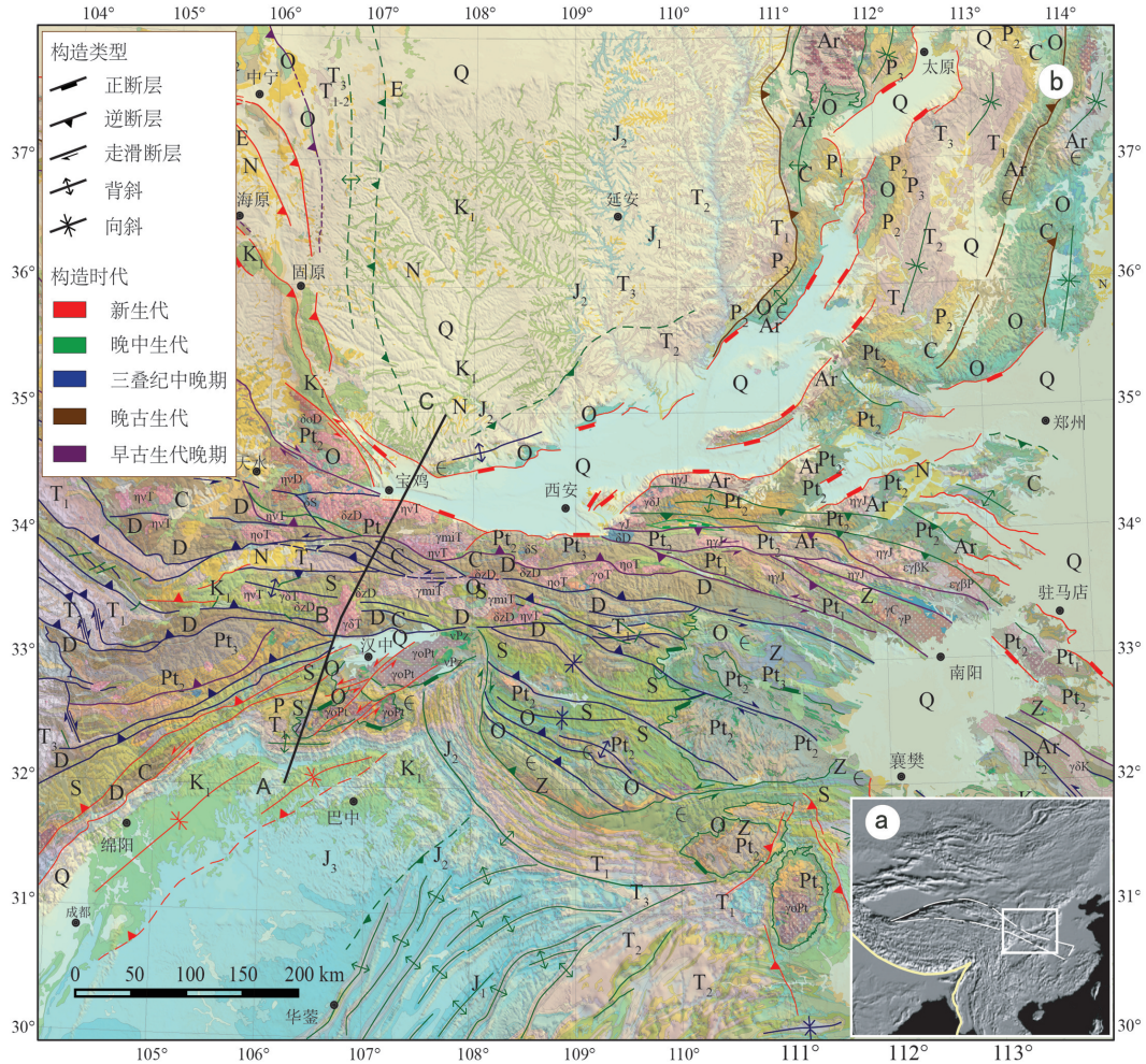
图1 研究区区域地质图 (地层代号及时代以中国地层表2014版为准) Fig. 1 Geological map of the study area (Geological legends after Chronostratigraphic Chart in China, 2014)
