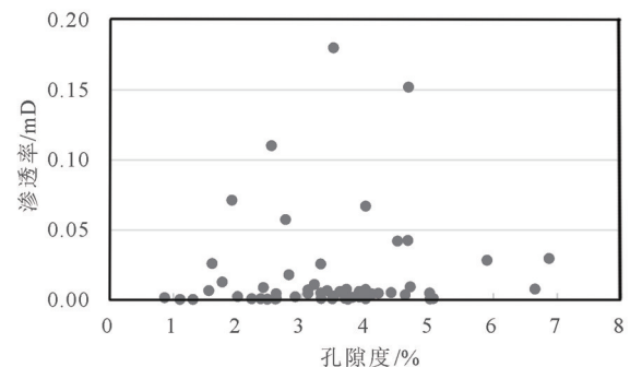
图4 研究区龙马溪组页岩孔隙度-渗透率散点图 Fig.4 Scatter diagram of porosity and permeability in shales of Longmaxi Formation in study area
