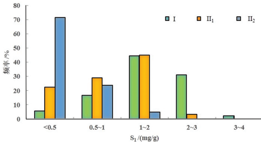
图12 不同有机质类型泥岩 S_1 含量分布 Fig.12 The S_1 content of different organic matter types of K_2qn_1
