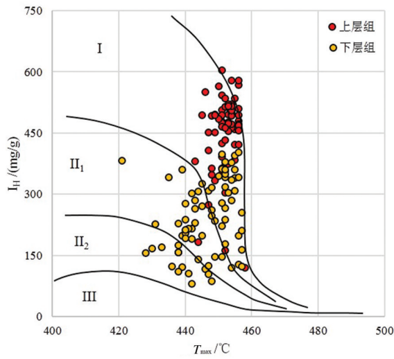
图10 青一段泥岩有机质类型判别图 Fig.10 The discrimination diagram of organic matter type of the mudstone of K_2qn_1
