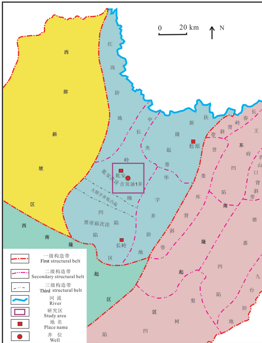
图1 研究区构造单元划分图 Fig.1 Structural map of southern Songliao Basin
