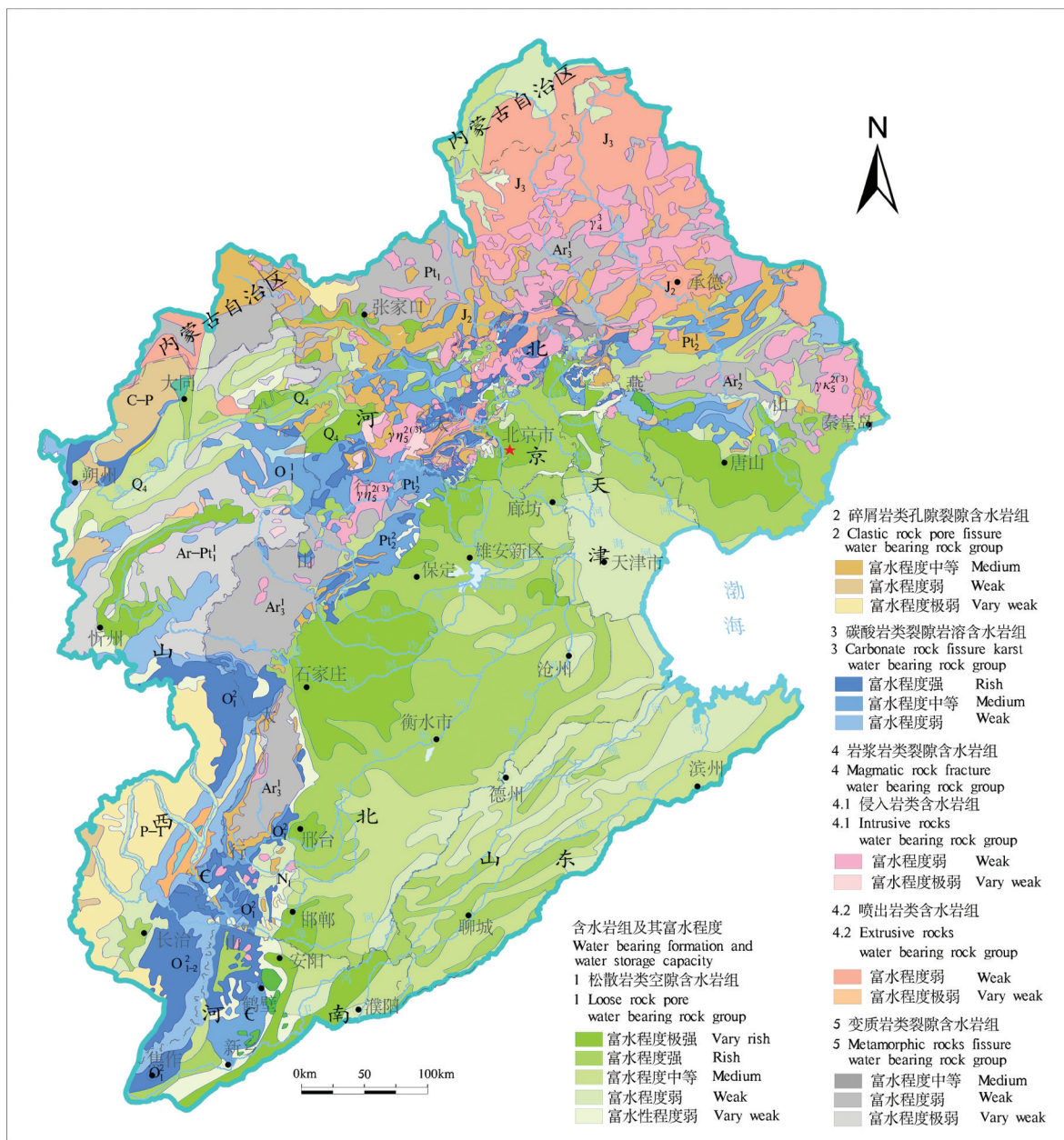
图2 海河流域水文地质图 Fig.2 Hydrogeological map of the Haihe River Basin
