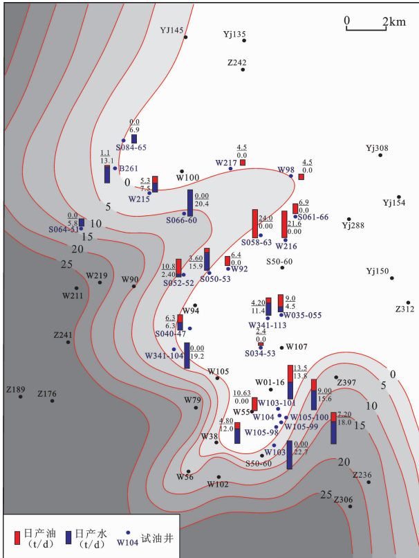
图6 吴堡地区长 8 1 烃源岩与试油产量关系图 Fig.6 Distribution of Chang-8 1 source rock and oil test yield in Wubao area
