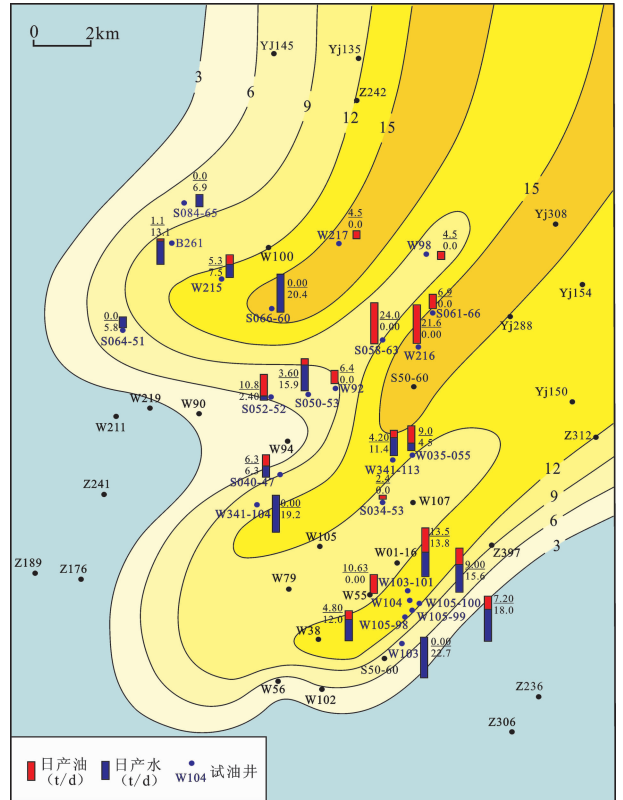
图7 吴堡地区长 8 1 砂体厚度与试油产量叠合图 Fig.7 Distribution of sand thickness and oil test yield of Chang-8 1 member in Wubao area
