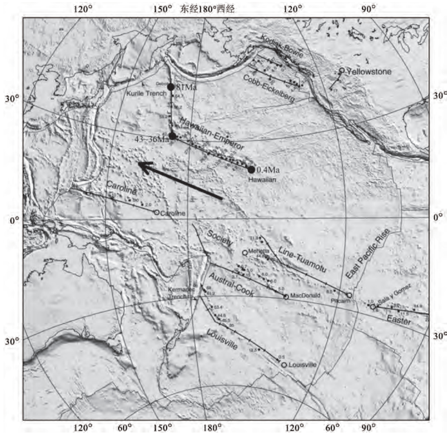
图14 夏威夷-皇帝海岭拐点标志着太平洋板块始新世—渐新世末的运动转向(据[41]改编) Fig.14 Pacific plate movement steering during Eocene-Oligocene marked by Hawaiian-Emperor ridge inflection point (modified after [41])
