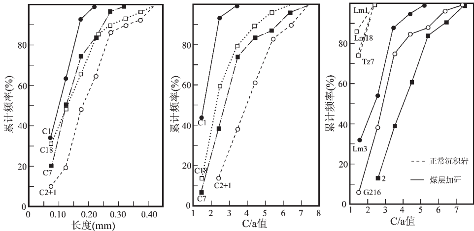
图1 滇东黔西地区宣威组中煤层夹矸和正常沉积粘土岩中锆石形态参数累积频率图(据周义平,1992) Fig. 1 Cumulative frequency diagram of zircon morphology parameters in dirt bands of coal beds and normal sedimentary claystone in the Dingwei Formation in the eastern Yunnan-western Guizhou area (C/a值:锆石的长度/宽度)
