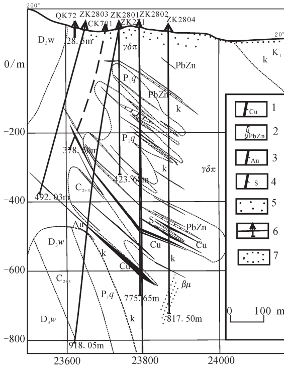
图19 安徽姚家岭铜铅锌矿28线剖面图(据蒋其胜,2006) 1—铜矿体;2—铅锌矿体;3—金矿体;4—硫矿体;5—高岭石化、黄铁矿化;k—钾长石化;6—钻孔;7—推测地质界线;K 1 —下白垩统火山碎屑岩;P 1 q—下二叠统栖霞组灰岩;C 2+3 —中上石炭统灰岩; D 3 w—上泥盆统五通组砂岩;γδπ—花岗闪长斑岩 Fig.19 Geological section of exploratory profile No. 28 of the Yaojialing copper-lead-zinc deposit, Anhui (after Jiang, 2006). 1—Copper orebody;2—Lead-zinc orebody;3—Gold orebody;4—Sulfur orebody;5—Kaolinization and pyritization;k—K-feldspar alteration;6—Borehole;7—Inferred geological boundary; K 1 —Lower Cretaceous Kedou Formation pyroclastic rocks; P 1 q—Lower Permian Xixia Formation limestone; C 2+3 —Middle-Lower Carboniferous limestone; D 3 w—Upper Devonian Wutong Formation sandstone; γδπ—granodiorite porphyry
