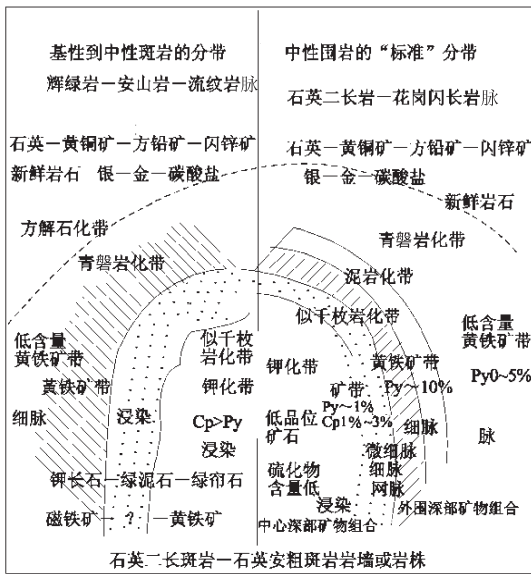
图15 斑岩铜矿的蚀变模式(引自胡惠民,1992) Fig.15 Alteration model of porphyry copper deposits (after Hu, 1992)
