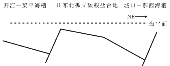
图10 孤立台地形态示意图 Fig.10 Diagrammatic map of the shape of the isolated platform
