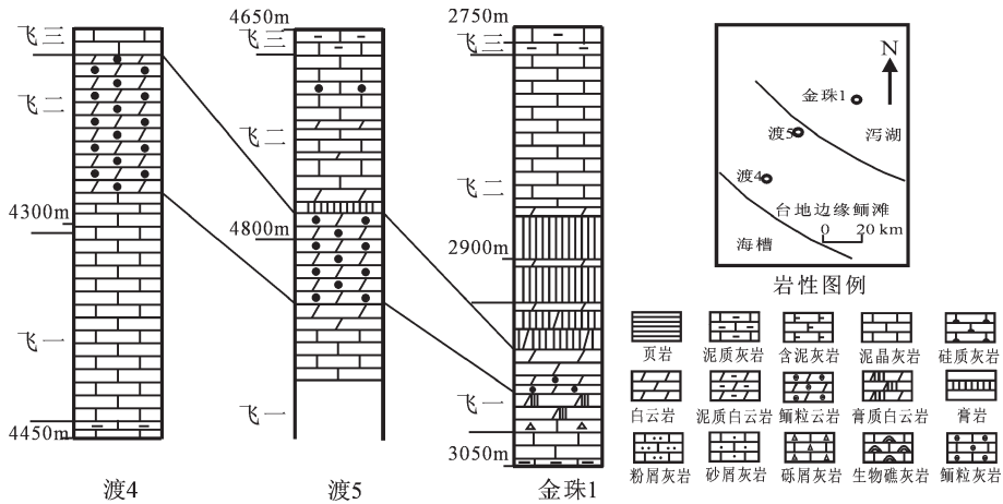
图9 渡4井—金珠1井储层对比图 Fig.9 Correlation of the reservoir shown by wells Du 4 to Jinzhu 1
