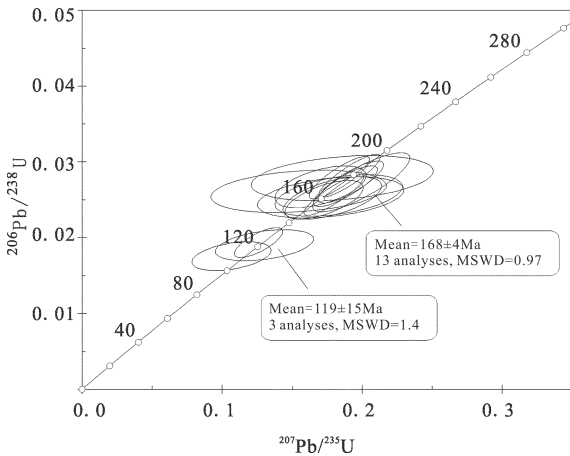
图3 紫金山黑云母花岗岩锆石 U-Pb 图解 Fig.3 SHRIMP U-Pb diagram of zircons from the Zijinshan biotite granite
