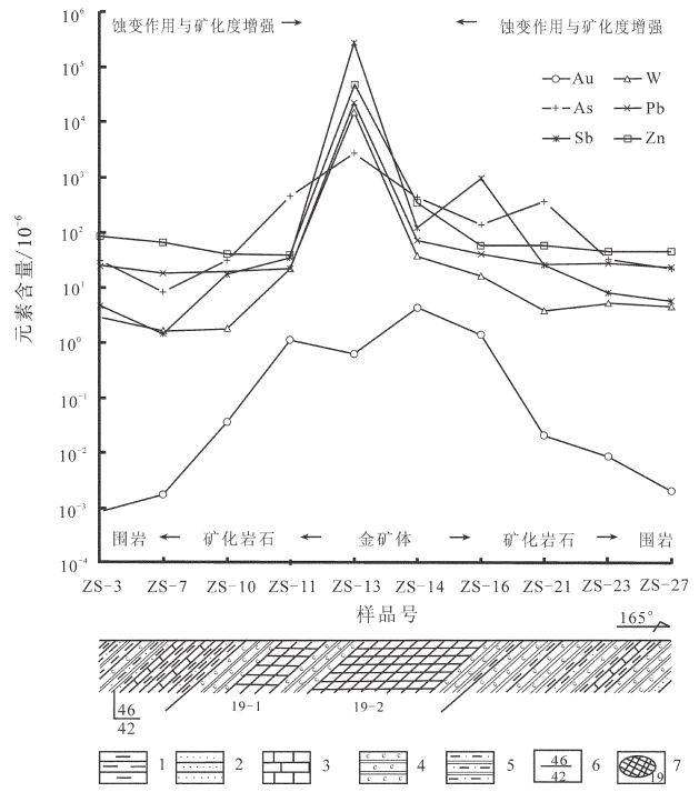
图 4 金矿床中 19 号矿体围岩、矿化岩石、矿石中 Au, W, Sb, As, Zn, Pb 含量变化及其与热液蚀变强度的关系 1—钙质板岩;2—粉砂岩;3—灰岩;4—炭质板岩;5—粉砂质板岩;6—地层产状;7—金矿体及编号 Fig.4 Variation of Au, W, Sb, As, Zn, Pb contents in ores, altered rocks and wall rocks as well as their correlation to alteration intensity 1—Calcareous slate;2—Silt sandstone;3—Limestone;4—Carbonaceous slate;5—Silty slate;6—Stratal attitude;7—Gold orebody and No
