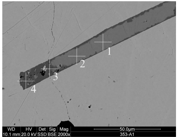
图 2 V3 矿脉中的硫锑铅矿(1,2)和车轮矿(3,4)矿物 Fig.2 SEM image showing the occurrence of boulangerite (1,2) and bourmonite(3,4) observed in V3 ore vein
