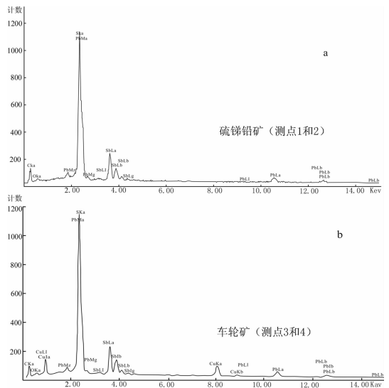
图 3 硫锑铅矿和车轮矿能谱曲线 Fig.3 EDS spectra patterns of boulangerite and bourmonite
