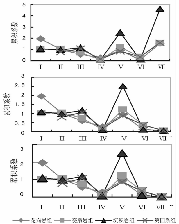
图 8 岩-土-脐橙系统中稀土元素累积系数变化趋势图 Fig.8 Changes in trends of REE accumulation factors in the rock-soil-avel orange system
