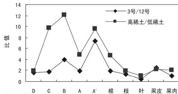
图 7 高、低稀土背景区岩土脐橙稀土含量差异趋势图 Fig.7 Differences in trends of REE content in rock-soil-avel orange in high-REE and low-REE background regions
