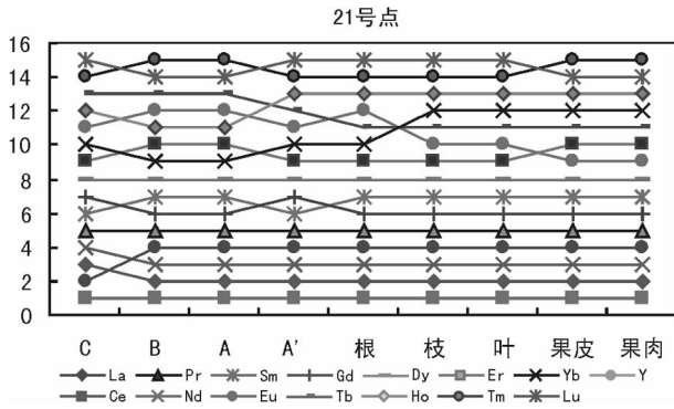
图 6 21 号点岩土脐橙系统中稀土元素百分比值次序图 Fig.6 Sequence of REE percentage in the rock-soil-avel orange system at sampling point 21
