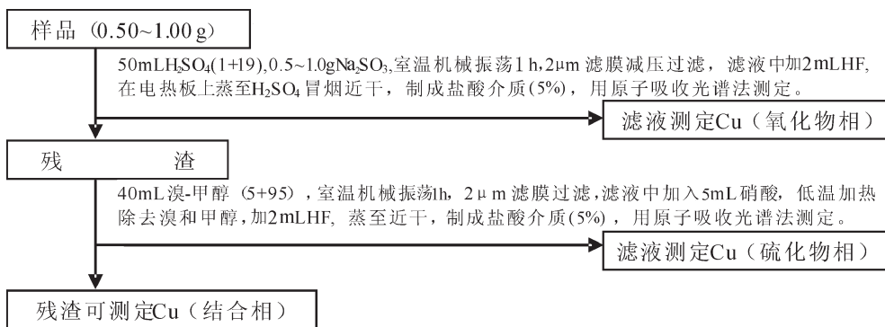
图 15 痕量铜元素相态提取、分析流程 Fig.15 Flow chart for phase extraction and analysis of trace copper
