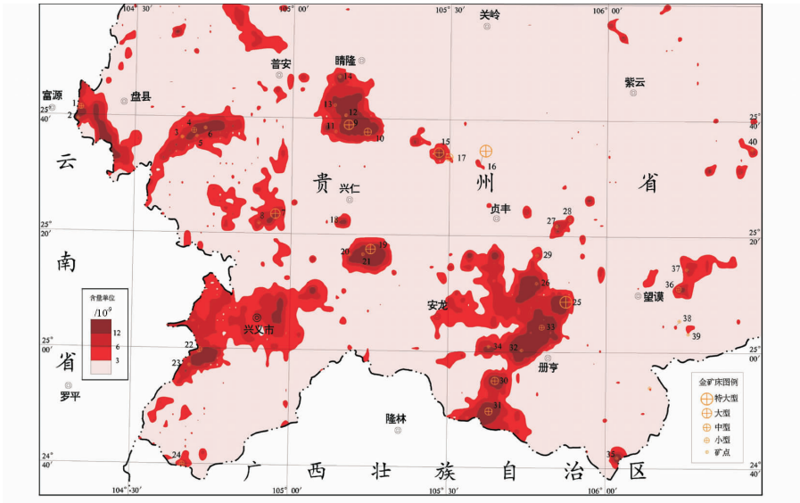
图 12 黔西南金异常及已发现金矿床位置图 Fig.12 Gold anomalies and gold deposits in southwestern Guizhou
