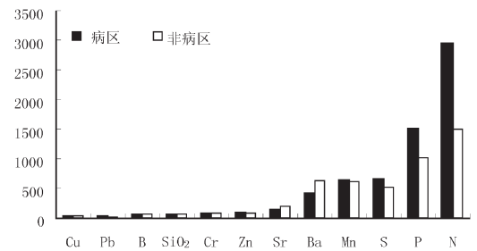
图 6 若尔盖县病区与非病区土壤化学成分关系(单位： \mu g/g ) Fig.6 Soil chemical composition comparison between the disease area and the non-disease area of Zoige County
