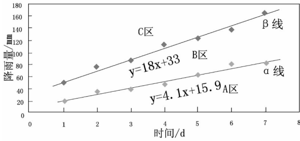
图4 灵台县 I 级预警区地质灾害气象预警预判判据模式图 Fig.4 Geological hazards meteorological early-warming criteria chart of Grade-I warning zone in Lingtai County
