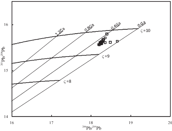
图2 锡铁山矿床基于铅同位素演化的 ^{207}\text{Pb}/^{204}\text{Pb} - ^{206}\text{Pb}/^{204}\text{Pb} 图解 Fig.2 ^{207}\text{Pb}/^{204}\text{Pb} versus ^{206}\text{Pb}/^{204}\text{Pb} diagram
