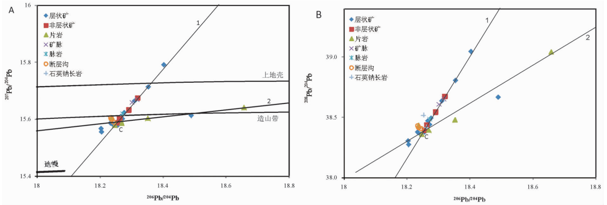
图3 锡铁山矿床铅同位素图解 (A 中的演化曲线参考自 Zartman and Doe 等 [16] ) Fig.3 Lead isotope diagram of the Xitieshan ore deposit (model curves from the Plumbotectonics model [16] )
