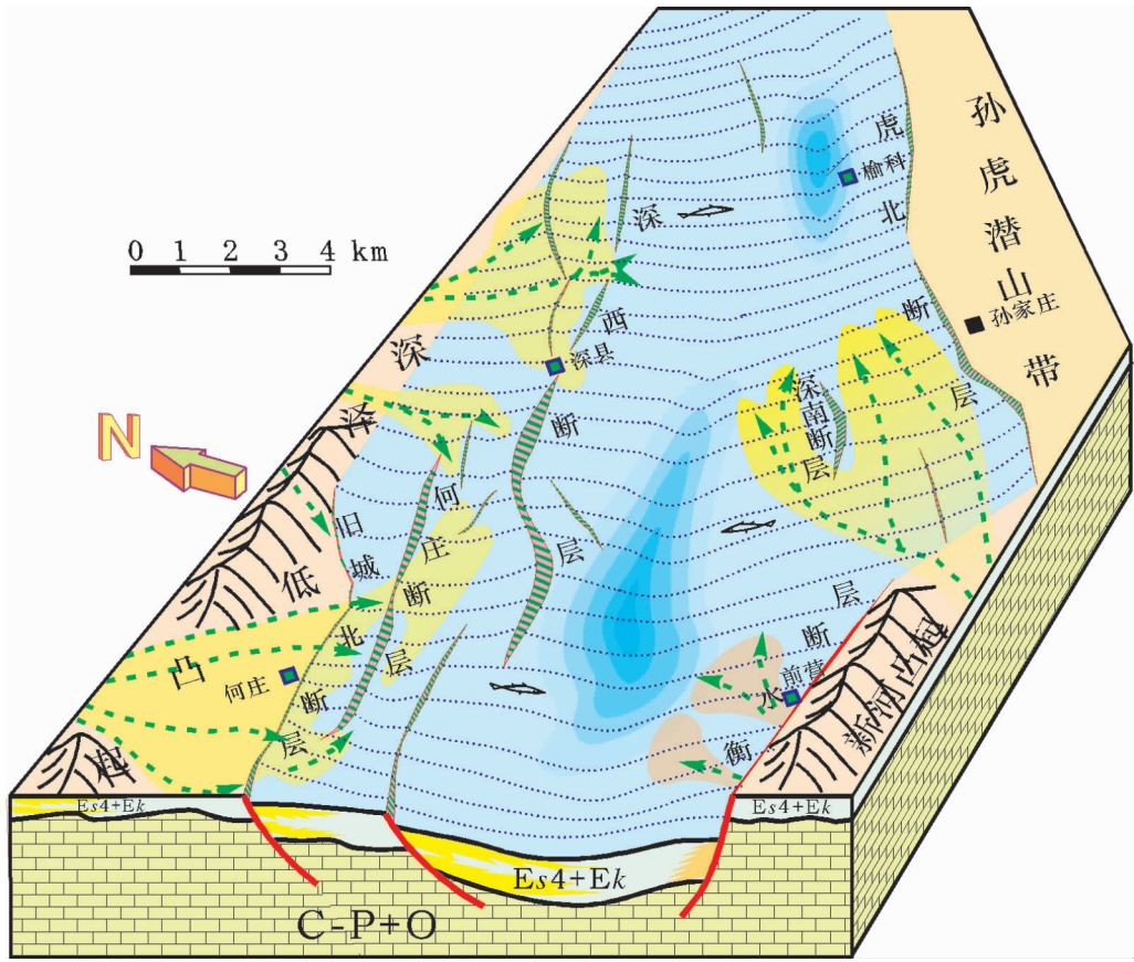
图 5 深县凹陷的古近系构造格局与沉积体系模式图 Fig.5 Model of Paleogene structural configuration and depositional system in Shenxian depression
