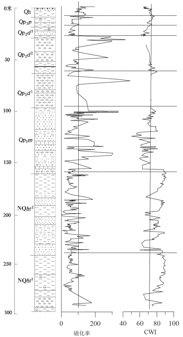
图 2 ZKC1 孔磁化率(10-6 SI)和化学风化指数(CWI)曲线 NQht 1 —上新世—早更新世华田组下段;NQht 2 —华田组上段; Qp 1m —早更新世汨罗组;Qp 2d 1 —中更新世洞庭湖组下段; Qp 2d 2 —洞庭湖组中段;Qp 2d 3 —洞庭湖组上段; Qp 3p —晚更新世坡头组;Qh—全新统 Fig.2 Curves of magnetic susceptibility (10-6 SI) and chemical weathering index (CWI) variation of ZKC1 borehole NQht 1 —Lower part of Pliocene—Early Pleistocene Huatian Formation; NQht 2 —Upper part of Huatian Formation; Qp 1m —Early Pleistocene Miluo Formation; Qp 2d 1 —1st part of Middle Pleistocene Dongtinghu Formation; Qp 2d 2 —2nd part of Dongtinghu Formation; Qp 2d 3 —3rd part of Dongtinghu Formation; Qp 3p —Late Pleistocene Potou Formation; Qh—Holocene
