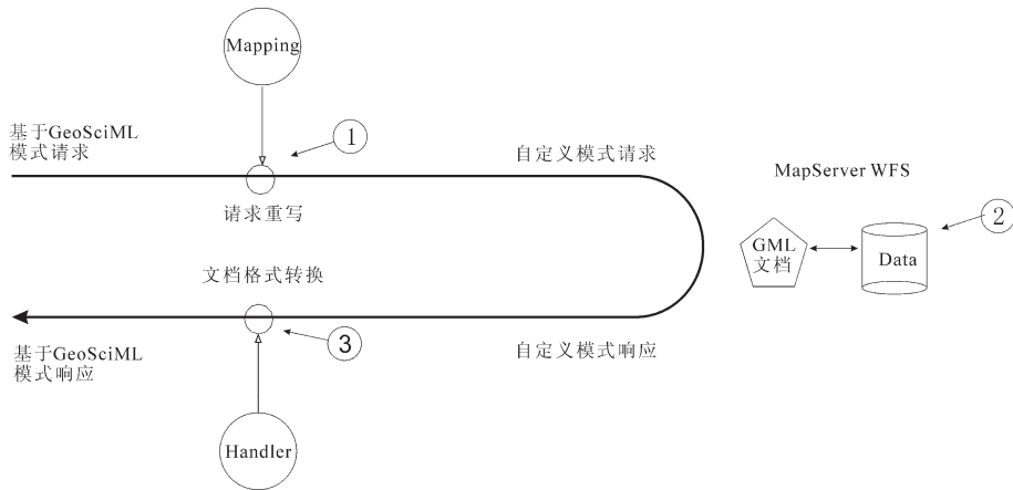
图 8 GeoSciML 网络要素服务 Fig.8 Web Feature Service based on GeoSciML
