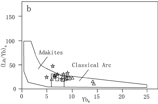
图 4 Y-Sr/Y(a)及 Yb N -(La/Yb) N (b)图解(图据文献[24]) Fig.4 Y-Sr/Y and Yb N versus (La/Yb) N diagram of intrusive rocks (after[24])
