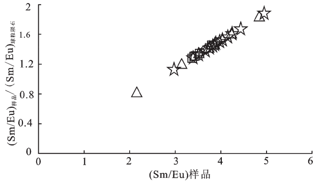
图 5 Sm/Eu-(Sm/Eu)样品/(Sm/Eu)球粒陨石图解(图例同图 4a) Fig.5 Diagram of (Sm/Eu) sample versus. (Sm/Eu) sample/ (Sm/Eu) condrite ( legends as for Fig. 4a)
