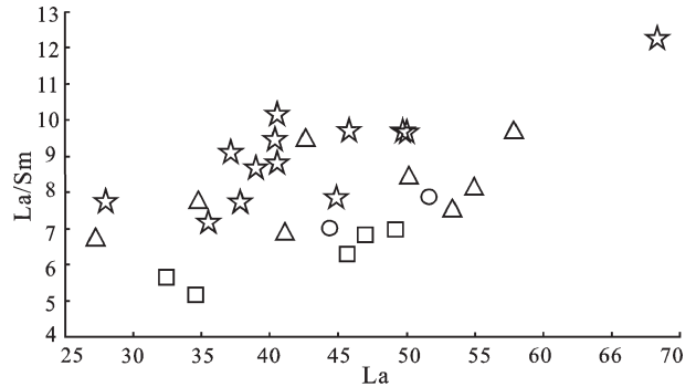
图 6 La-La/Sm 图解(图例同图 4a) Fig.6 Diagram of La versus La/Sm (legends as for Fig. 4a)
