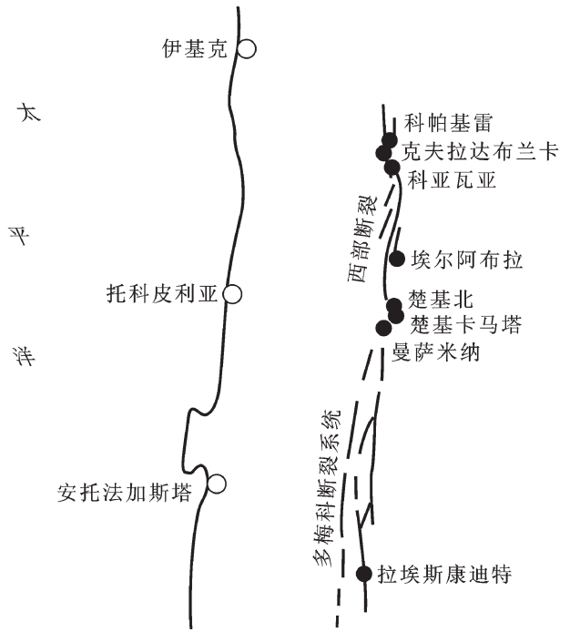
图2 智利楚基卡马塔铜矿床区域构造示意图 Fig.2 Regional tectonic diagram of the Chu Kika Mata Cu deposit in Chile
