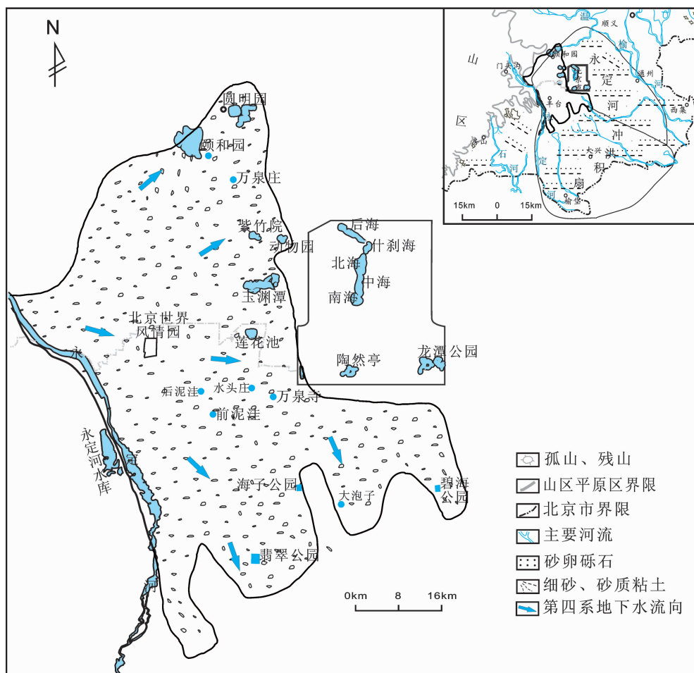
图3 北京城湖泊展布与单一砂砾石层分布图(据刘则制内部资料修编) Fig.3 The distribution of lakes and sand and gravel layers in Beijing plain
