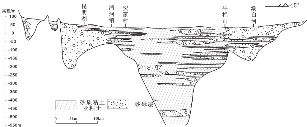
图 4 昆明湖附近地质剖面示意图 Fig.4 Geological cross section of the vicinity of the Kunming Lake
