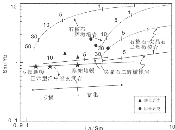
图12 La/Sm-Sm/Yb图解(文献[39])
