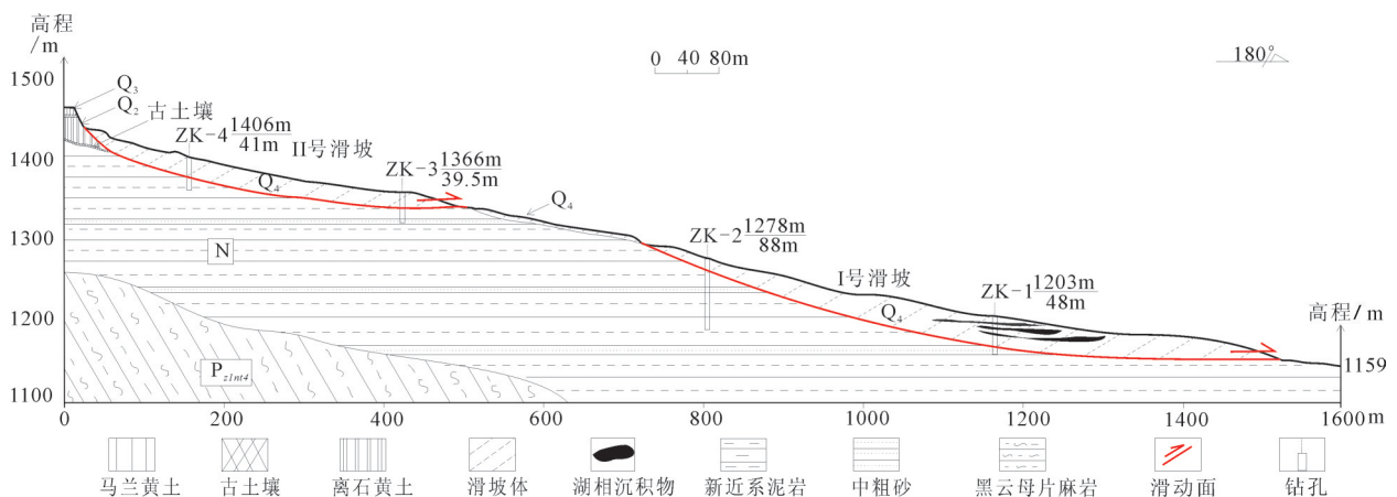
图4 红旗山滑坡工程地质剖面图 Fig.4 Engineering geological profile of Hongqishan landslide
