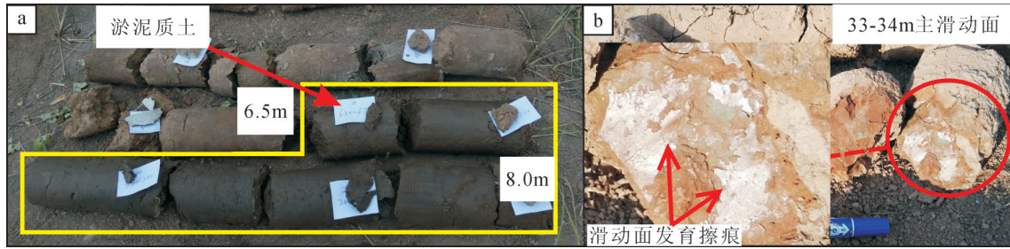
图6 红旗山滑坡钻孔岩心 a—ZK1 孔 6.5~8.0m 揭露的黑色湖相沉积物; b—ZK1 孔揭露滑动面 Fig.6 The photo of Hongqishan landslide cores a—Black lake sediments revealed by ZK1; b—Slip surface exposed by ZK1
