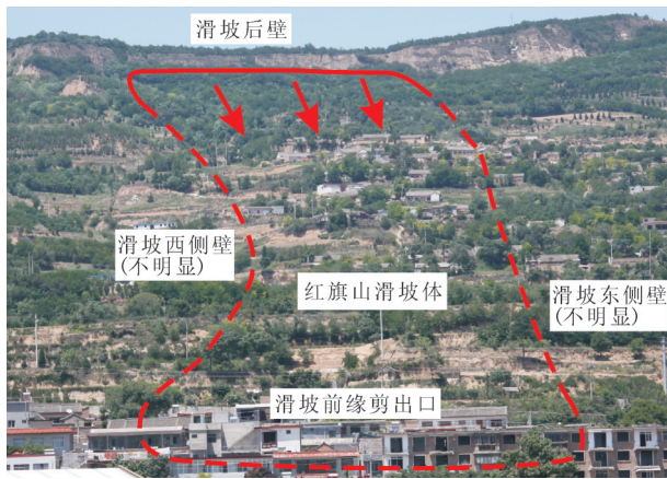
图3 红旗山滑坡全范围分布图 Fig.3 Full range distribution of Hongqishan landslide
