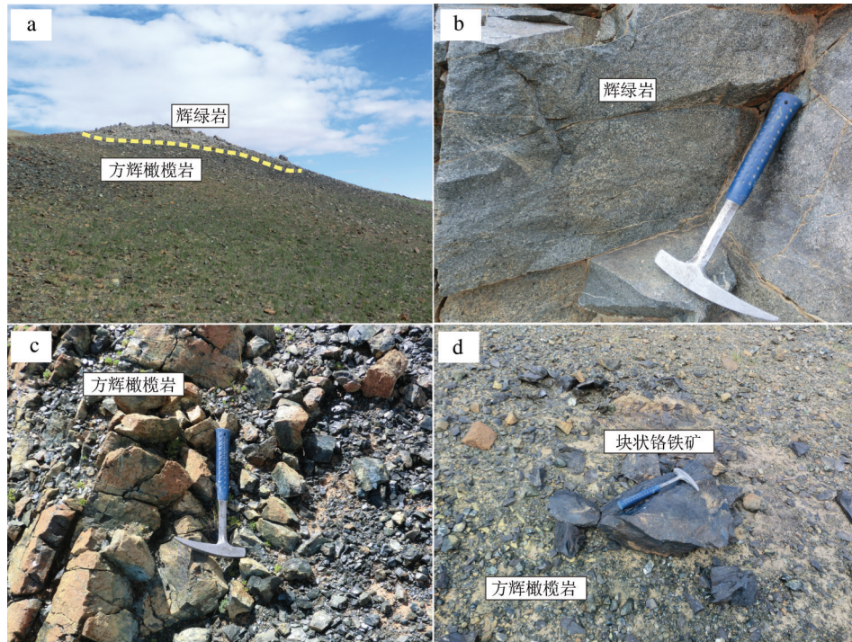
图3 雅鲁藏布江缝合带北亚带错不扎铬铁矿野外照片 Fig.3 Field relations and outcrops of the Cuobuzha chromitite.
