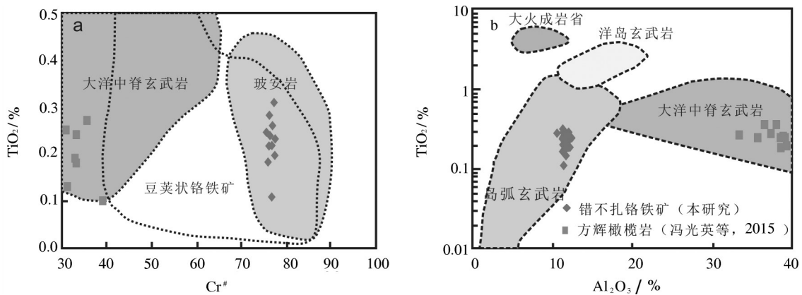
图7 错不扎铬铁矿和方辉橄榄岩中尖晶石的Cr # -TiO 2 (据Pagé and Barnes, 2009)和Al 2 O 3 -TiO 2 图解 (据Kamenetsky et al., 2001) Fig.7 Cr # - TiO 2 (after Pagé and Barnes, 2009)and Al 2 O 3 - TiO 2 diagrams (after Kamenetsky et al., 2001)of the Cuobuzha chromitite and harzburgite
