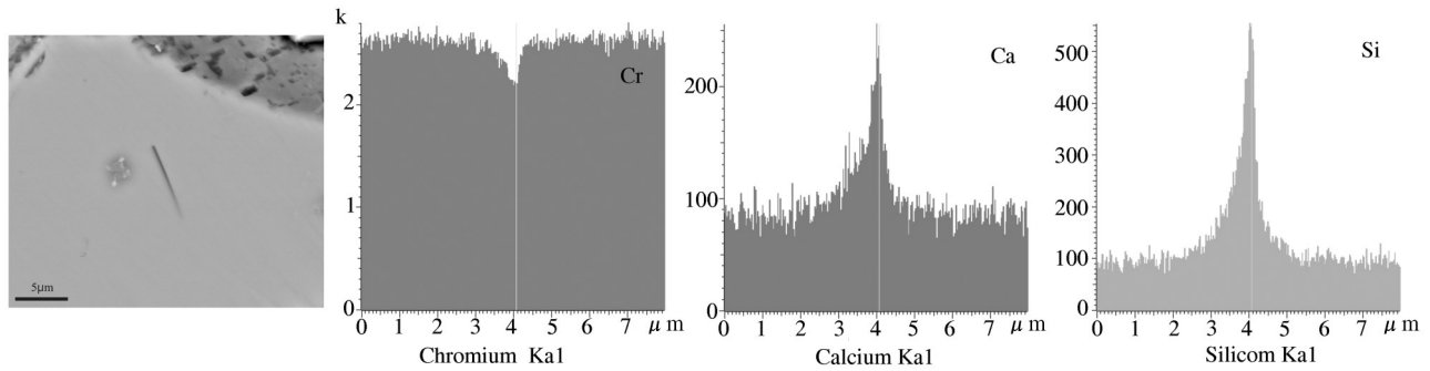
图6 错不扎铬铁矿铬尖晶石中单斜辉石出溶体成分扫描图 Fig.6 Compositional images of clinopyroxene exsolutions in chromites from the Cuobuzha chromitite
